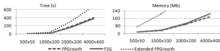
Fig.3: Efficiency of F2G and FPGrowth methods for datasets with varying size
