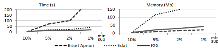
Fig.6: Efficiency of full-pattern mining methods for the yeast (2884×17) microarray
